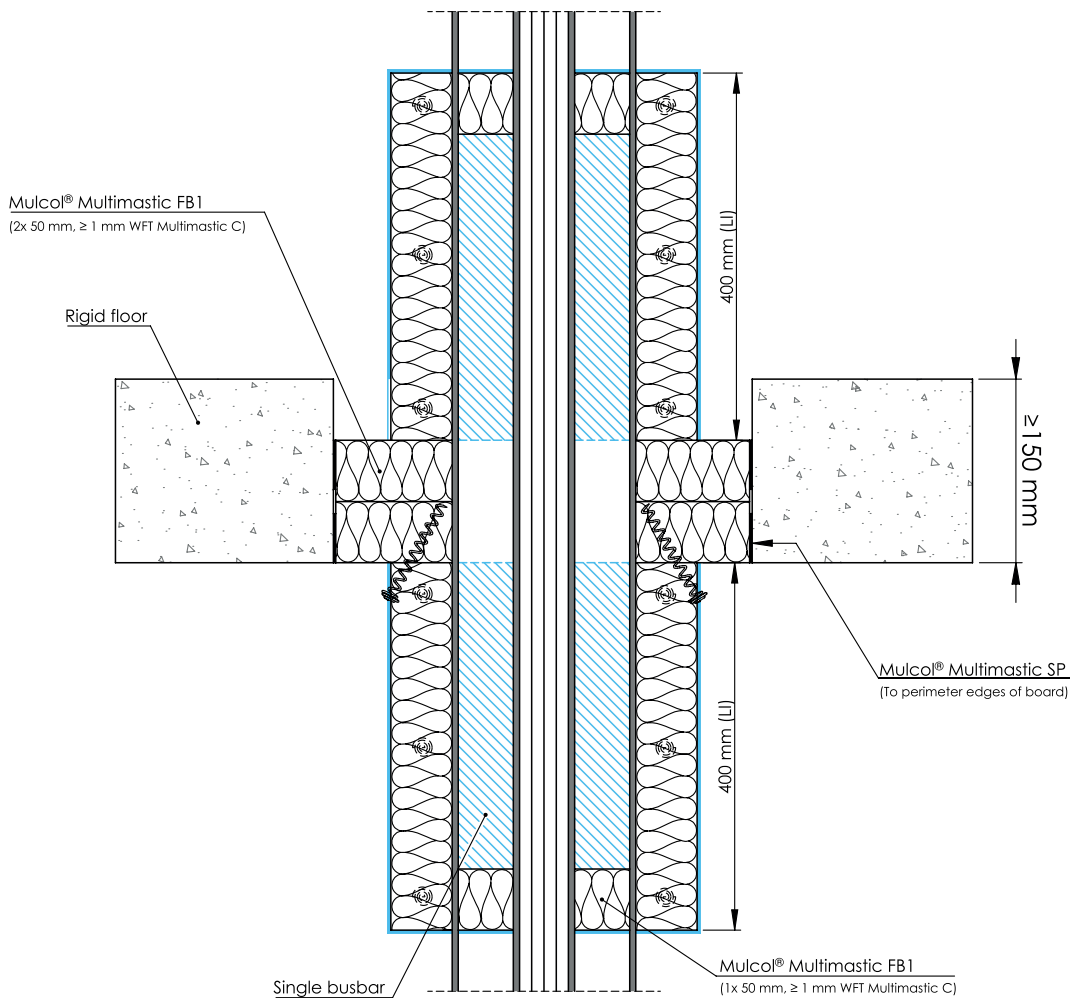
Drawing: PBrf.E-1BB-MFB1.2.10
