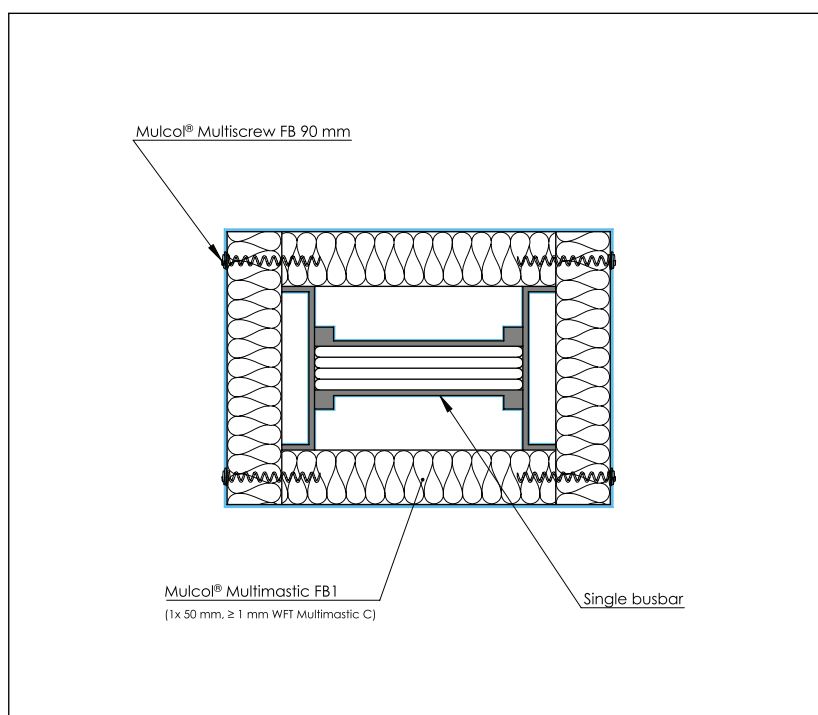
Front view
