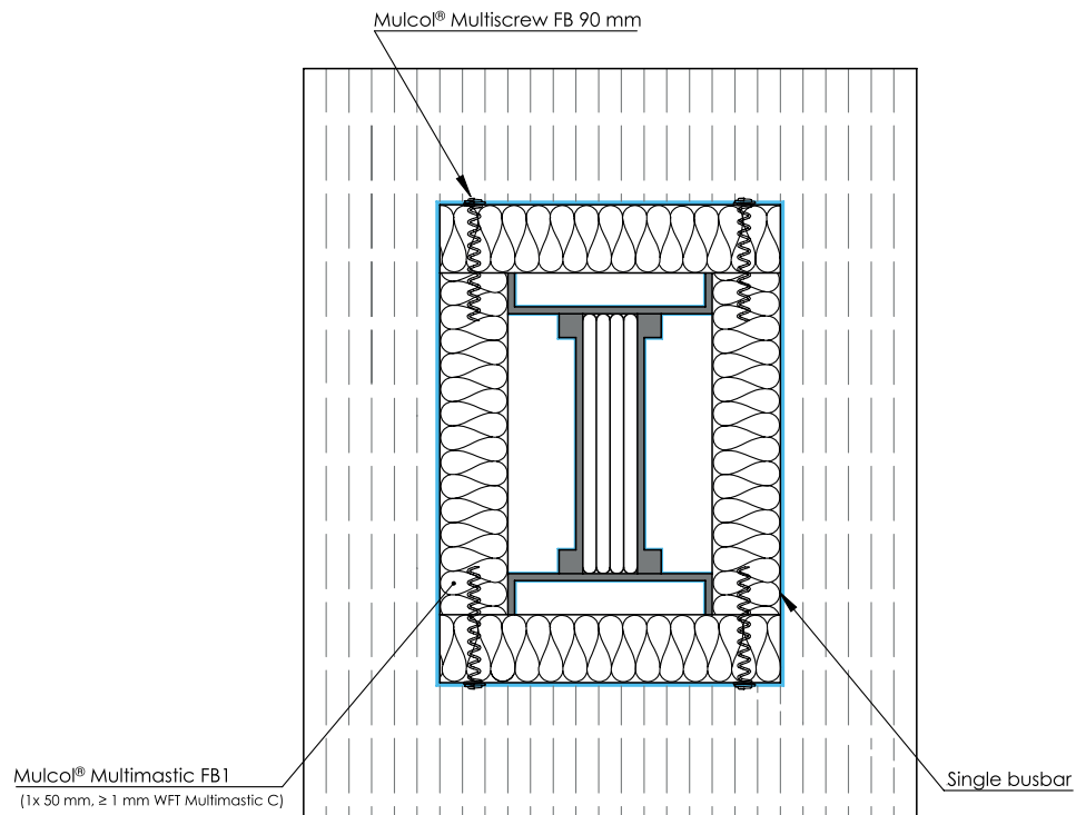
Bottom view
