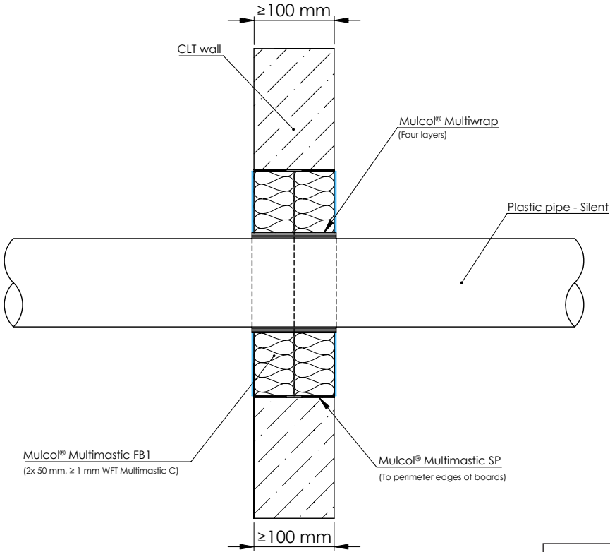
Drawing: WCLT-PPS-MW4-MFB1.2.10
