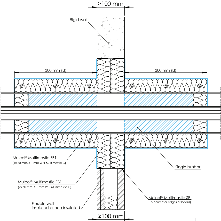
Drawing: PBfw.E-1BB-MFB1.2.10
